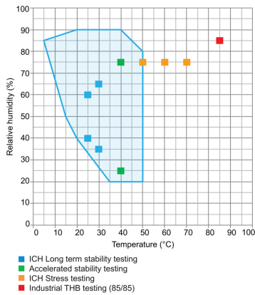
Climate chart
